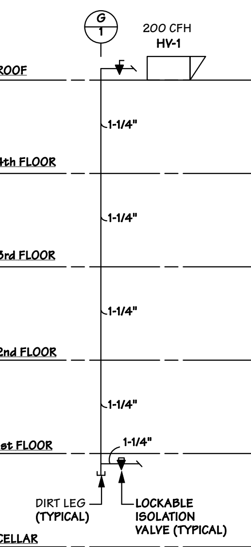
GAS RISER DIAGRAM NOT TO SCALE
